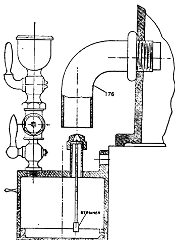
Sectional View of Starting Lamp Showing Burner and Blowpipe.
